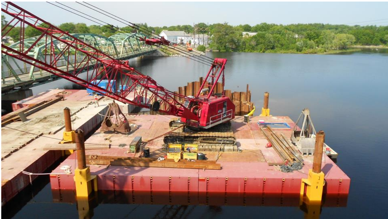
Photo 5: Example of a spud barge with crane, clamshell suited for this work.
