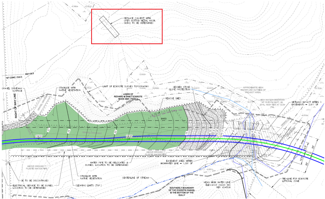
Figure 6-1: Location of the culvert to be replaced on the Eckrote parcel.
