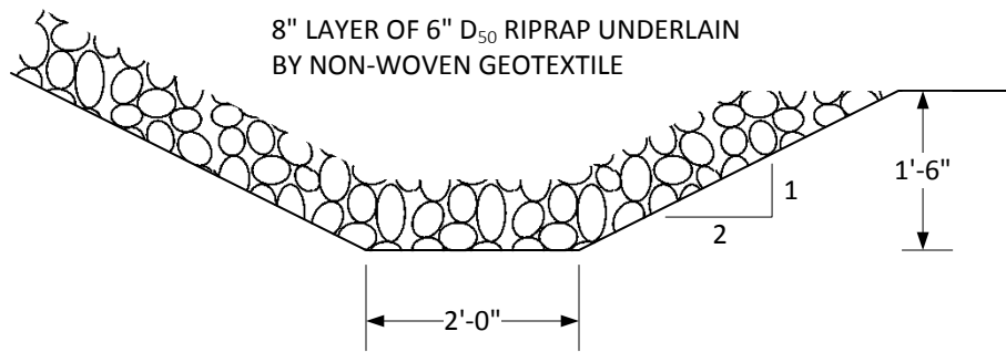
RIPRAP CHANNEL DETAIL
