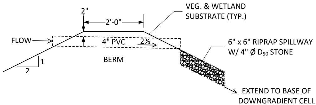
TRANSFER PIPE AND SPILLWAY DETAIL
