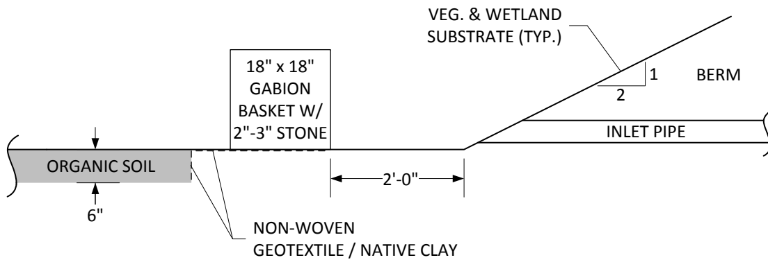
INLET FOREBAY DETAIL
