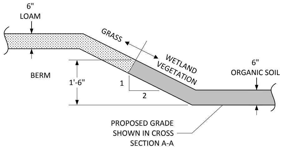
VEGETATION AND WETLAND SUBSTRATE DETAIL
