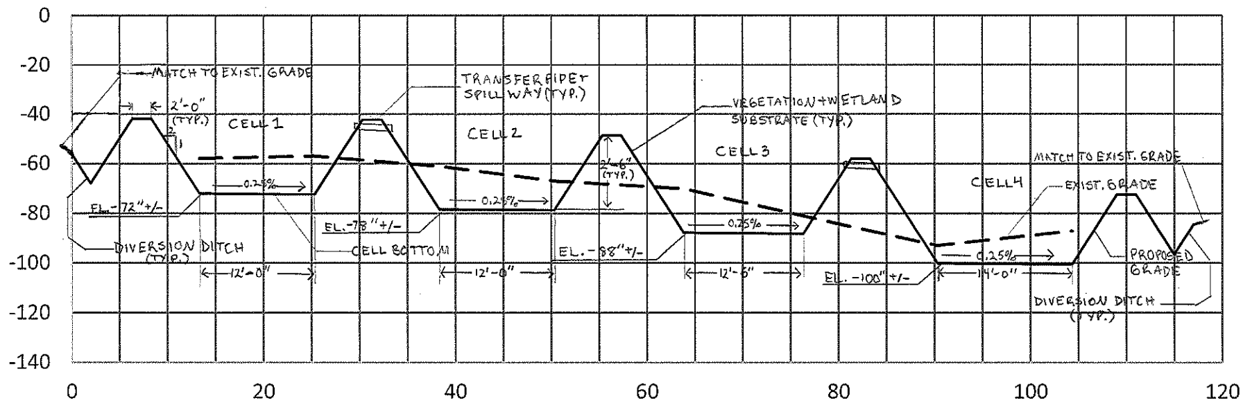
SECTION A HORZ. in feet VERT. in inches
