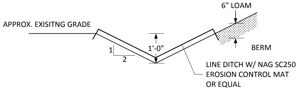
DIVERSION DITCH DETAIL
